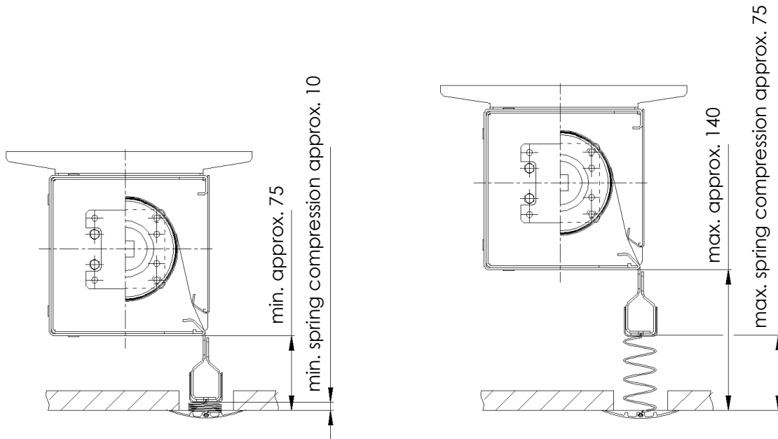
Fig. 5 Recommended position of casings relative to the ceiling. Gap width.
