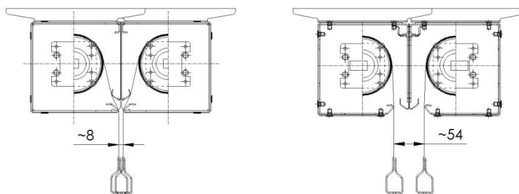
Fig. 19 Typical gap sizes in the transverse direction in the case of butt arrangement of curtains, type K, C and L casings.
