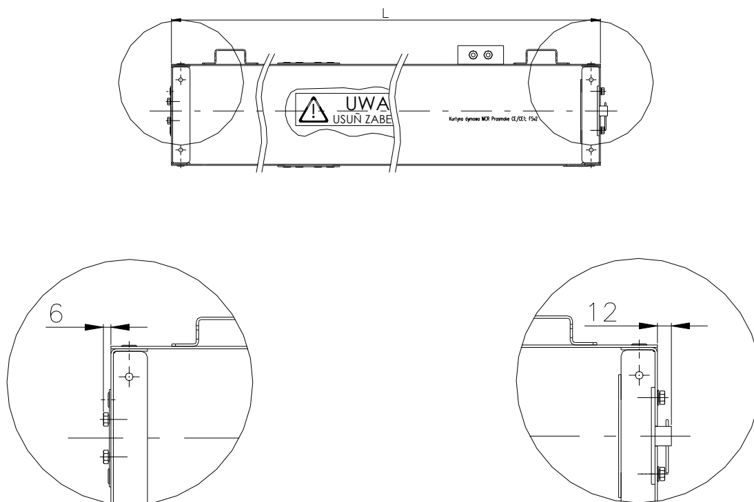
Fig. 2 Lengths of elements projecting beyond the mcr PROSMOKE FS CE curtain casing outline.
