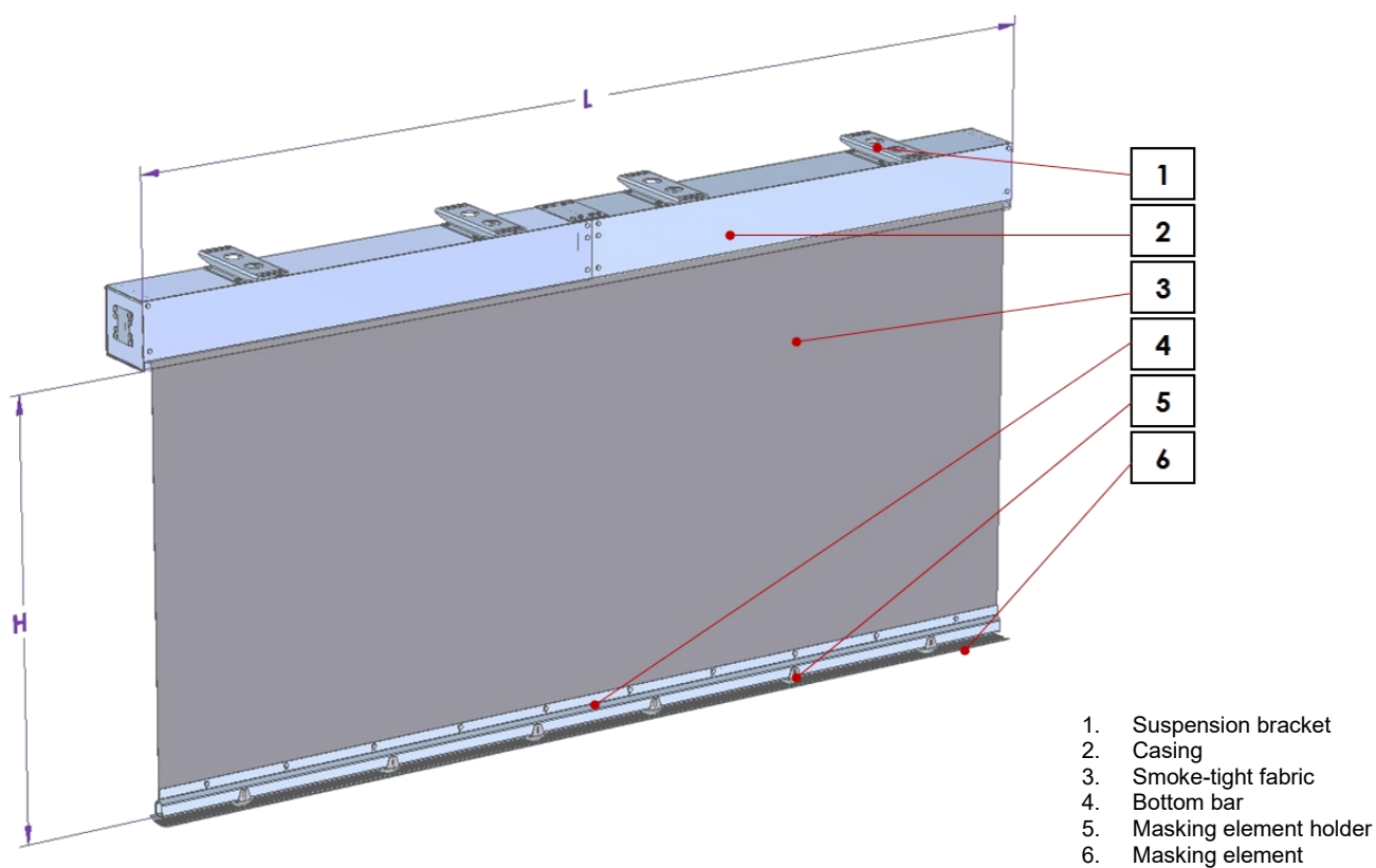
Fig. 1 mcr PROSMOKE FS CE rolling smoke curtain – design.
