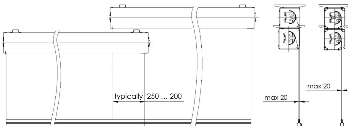
Fig. 14 Typical gap sizes in the transverse direction in the case of vertical arrangement of curtain modules with fabrics overlapping.
