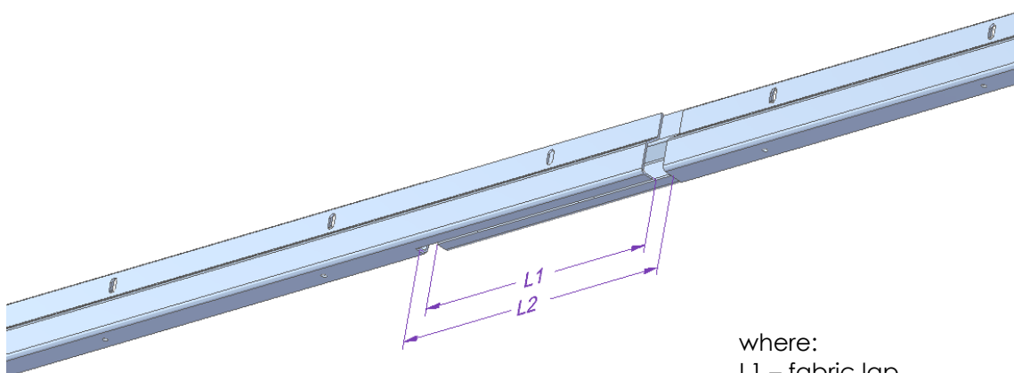
Fig. 20 Overlapping bottom bar – no connection of curtains by means of a common bottom bar.
