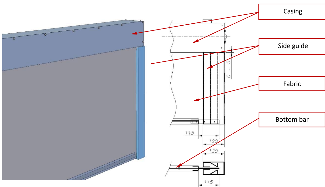
Fig. 23 Method of installing side guides.
