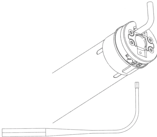
Fig. 7 Curtain limit switch adjustment.
