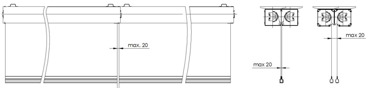
Fig. 17 Typical gap sizes in the transverse direction in the case of butt arrangement of curtain modules with type K, C and L casings and without fabrics overlapping.
