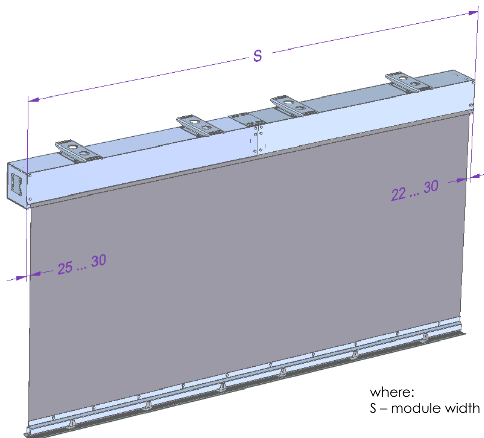
Fig. 21 Lengths of gaps in the longitudinal direction of mcr PROSMOKE FS CE curtains.
