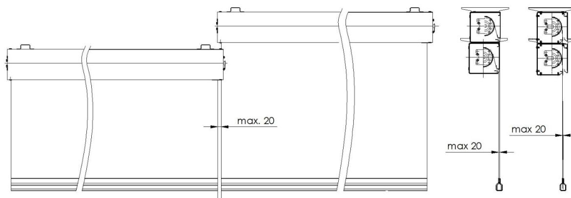
Fig. 15 Typical gap sizes in the transverse direction in the case of vertical arrangement of curtain modules without fabrics overlapping.
