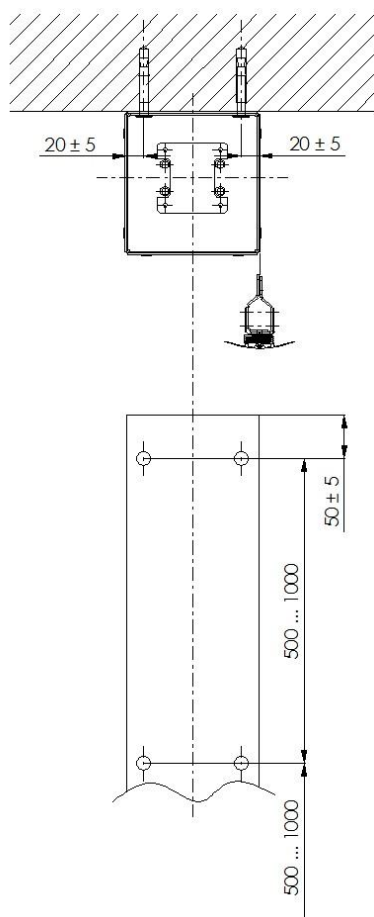
Fig. 9 Installation of a curtain without a suspension bracket.
