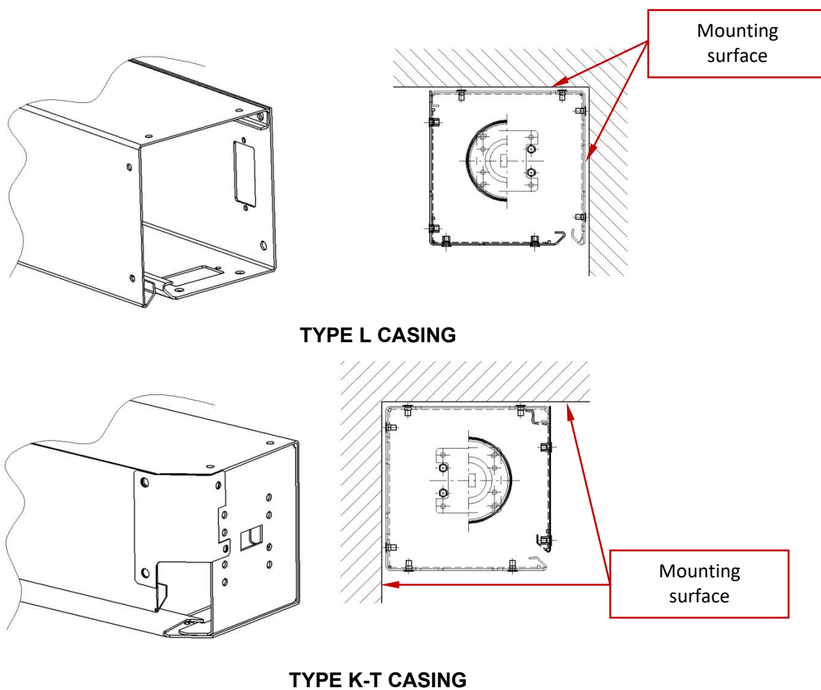
Fig. 4 Curtain casing types – L, K-T.
