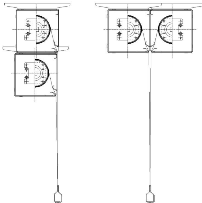
Fig. 18 Reduction in gaps in a group of curtains by using a common bottom bar – type F casings arranged vertically and horizontally.
