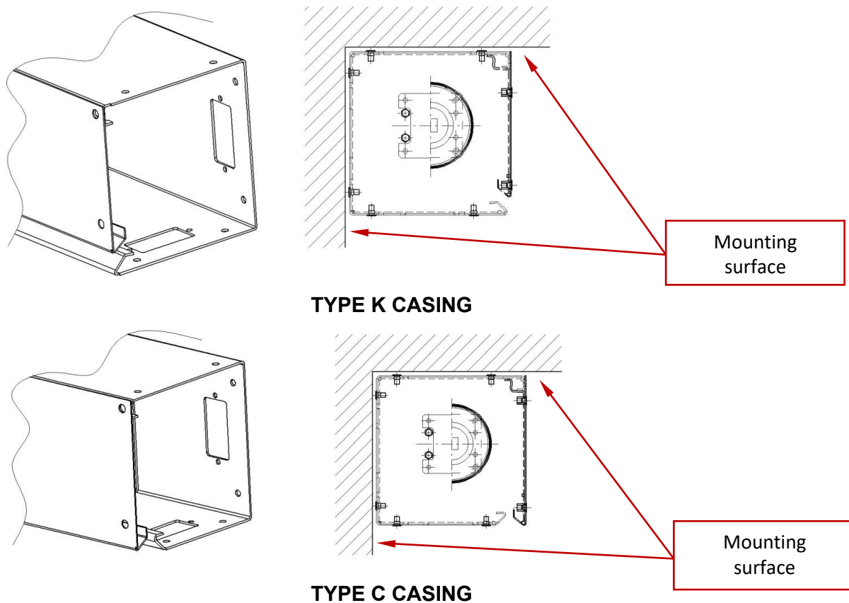
Fig. 3 Curtain casing types – K, C.
